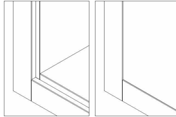
Flush System
